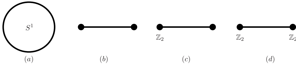
Figure 1: Compact connected 1-orbifolds
