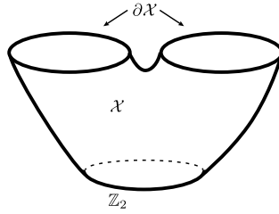
Figure 2: An orbifold X with only codimension 1 strata that does not retract to \partial X
